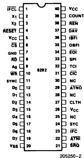
Figure 2. Pin Configuration
