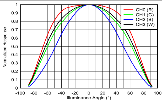
Figure 7-2. Device Response vs Illuminance Angle
