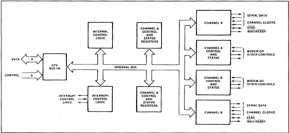
Figure 8 : Block Diagram.
